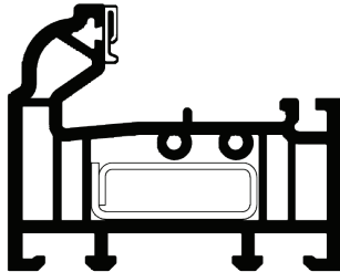
56MM PVC-U THRESHOLD (OVOLO)
