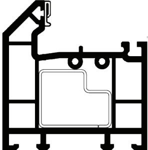
72MM PVC-U THRESHOLD (BEVELLED)
