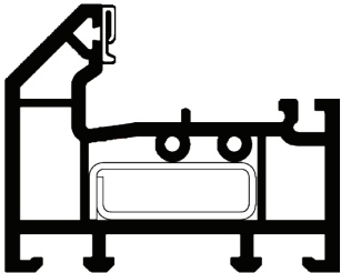
56MM PVC-U THRESHOLD (BEVELLED)
