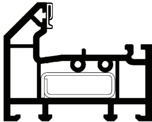
56MM PVC-U THRESHOLD (BEVELLED)
