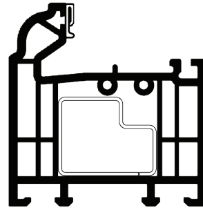
72MM PVC-U THRESHOLD (OVOLO)
