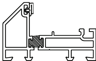
44MM ALUMINIUM THRESHOLD (BEVELLED)
