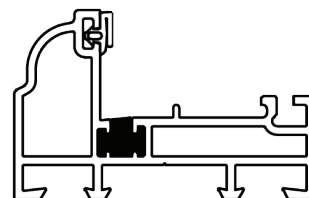
44MM ALUMINIUM THRESHOLD (OVOLO)
