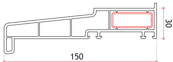
Flat Bed Cill 85mm, 150mm, 180mm
