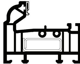
56MM PVC-U THRESHOLD (OVOLO)
