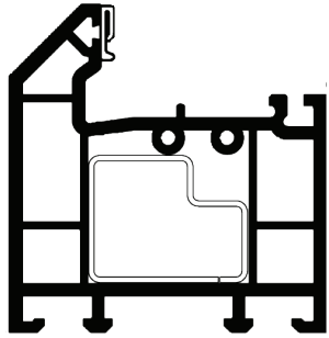
72MM PVC-U THRESHOLD (BEVELLED)
